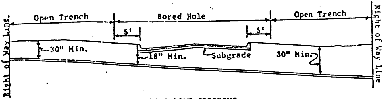
PIPE LINE CROSSING
