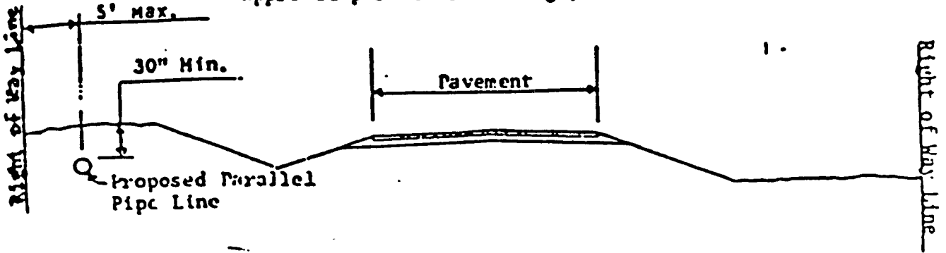
PARALLEL PIPE LINE
