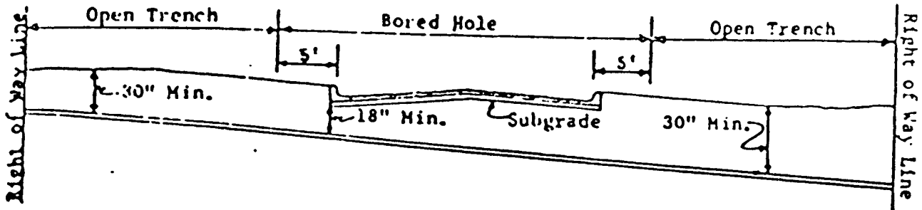
PIPE LINE CROSSING
