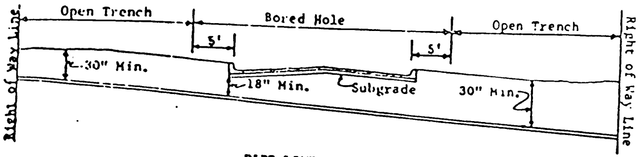
PIPE LINE CROSSING
