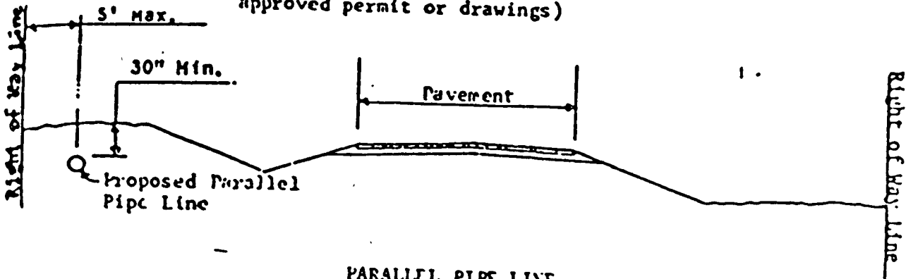
PARALLEL PIPE LINE
