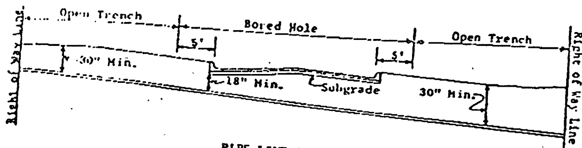
PIPE LINE CROSSING
